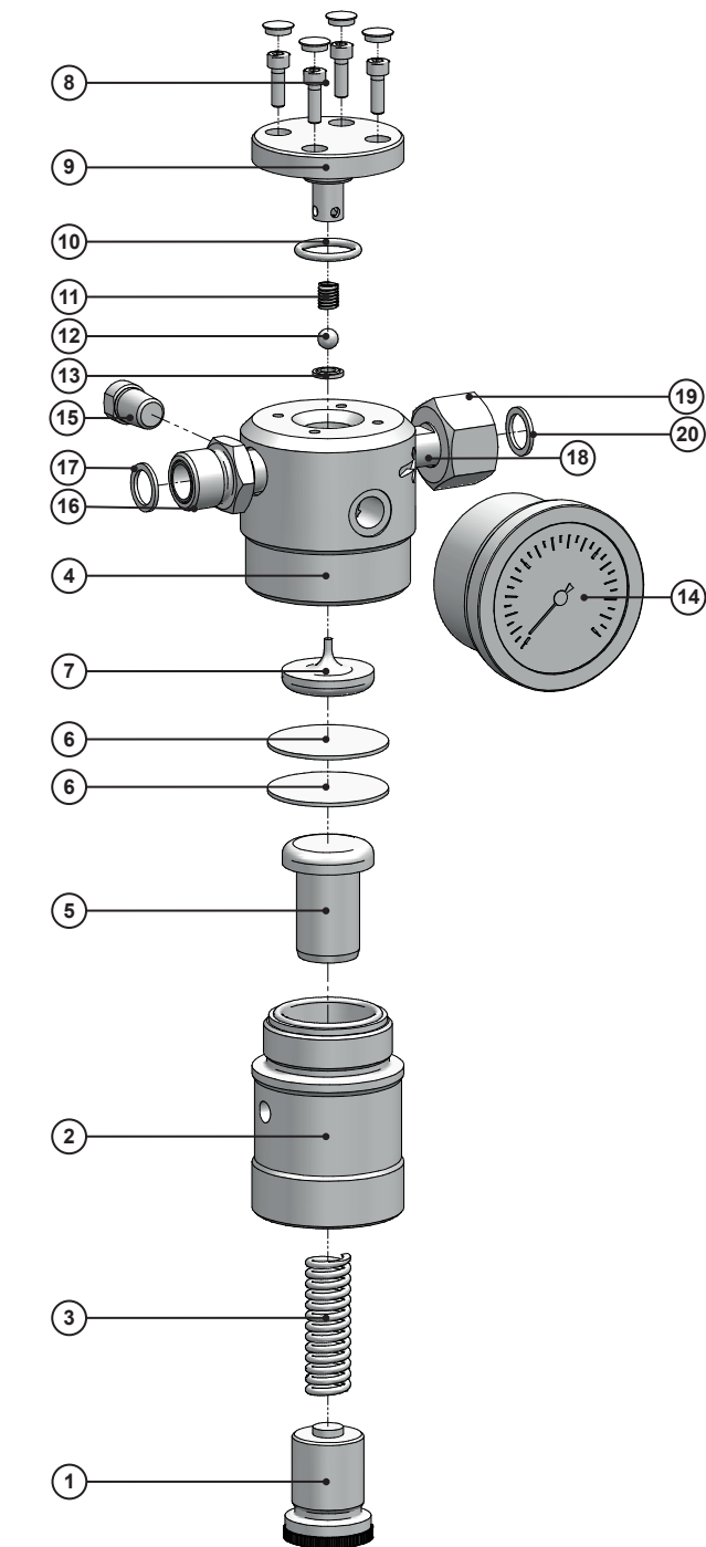
Fig. 13: Exploded view C 7105 pressure reducing valve
