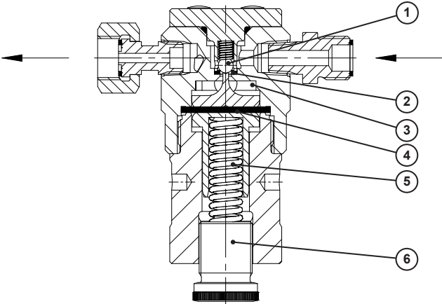
Fig. 1: Cross section C 7105
