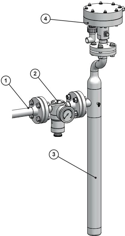
Fig. 2: Installation example C 7105 pressure reducing valve
