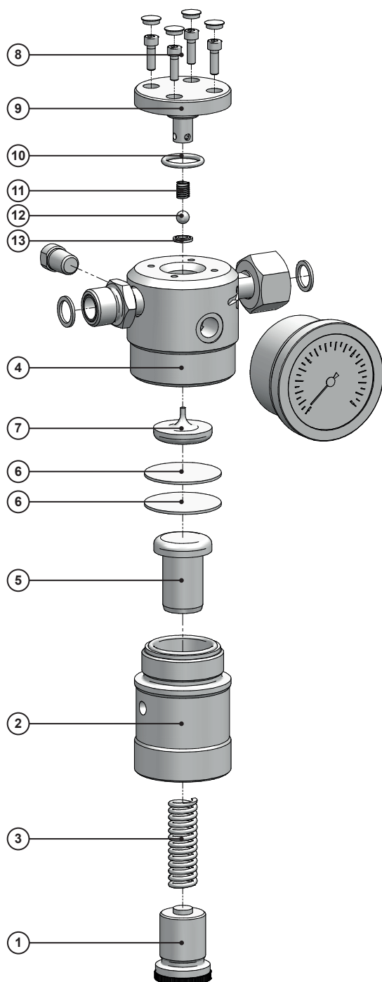
Fig. 12: Dismantle the device
