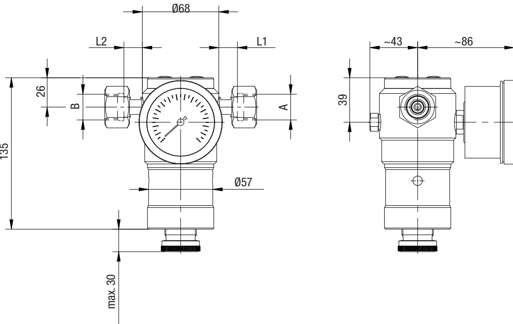
Fig. 8: Dimensional drawing C 7105 with union nuts
