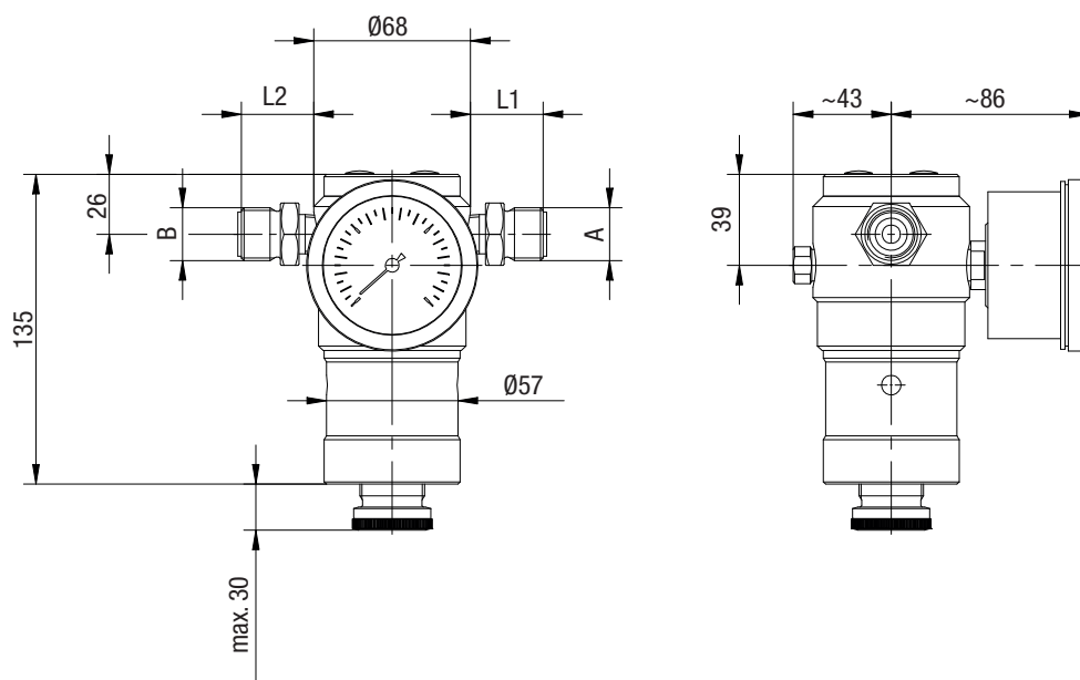
Fig. 6: Dimensional drawing C 7105 with threaded pin
