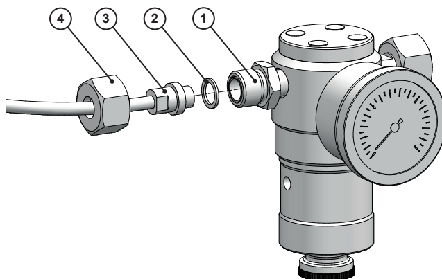
Fig. 9: Fitting the connection line
