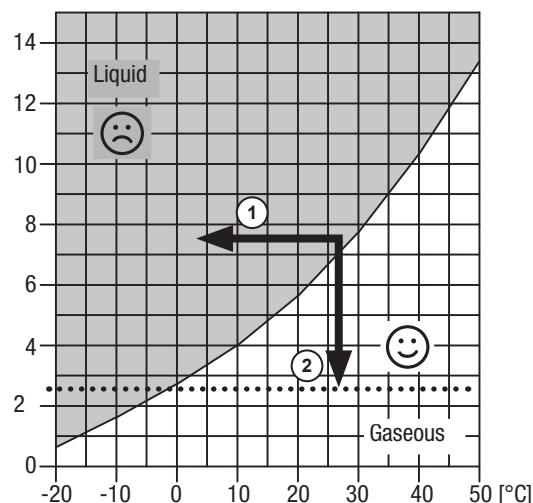
Fig. 3: Vapour pressure curve for chlorine
