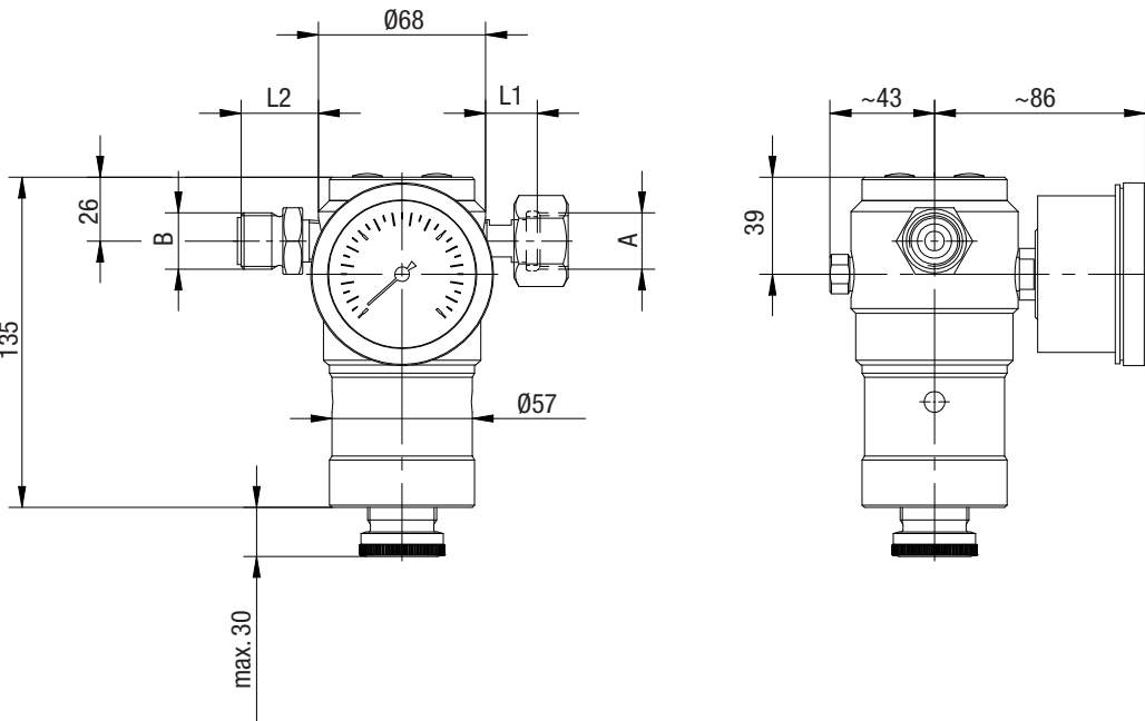
Fig. 7: Dimensional drawing C 7105 with threaded pin and union nut
