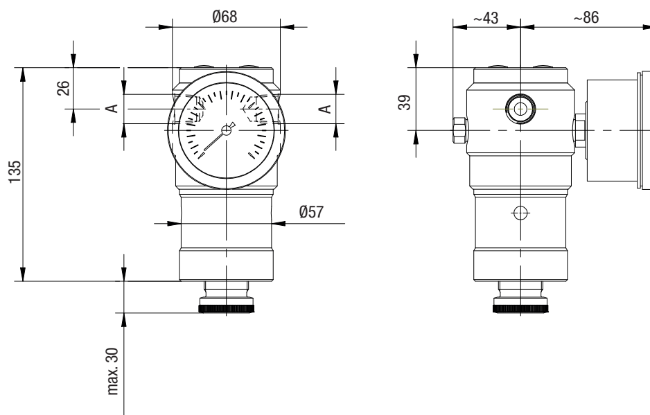
Fig. 5: Dimensional drawing C 7105 without connections
