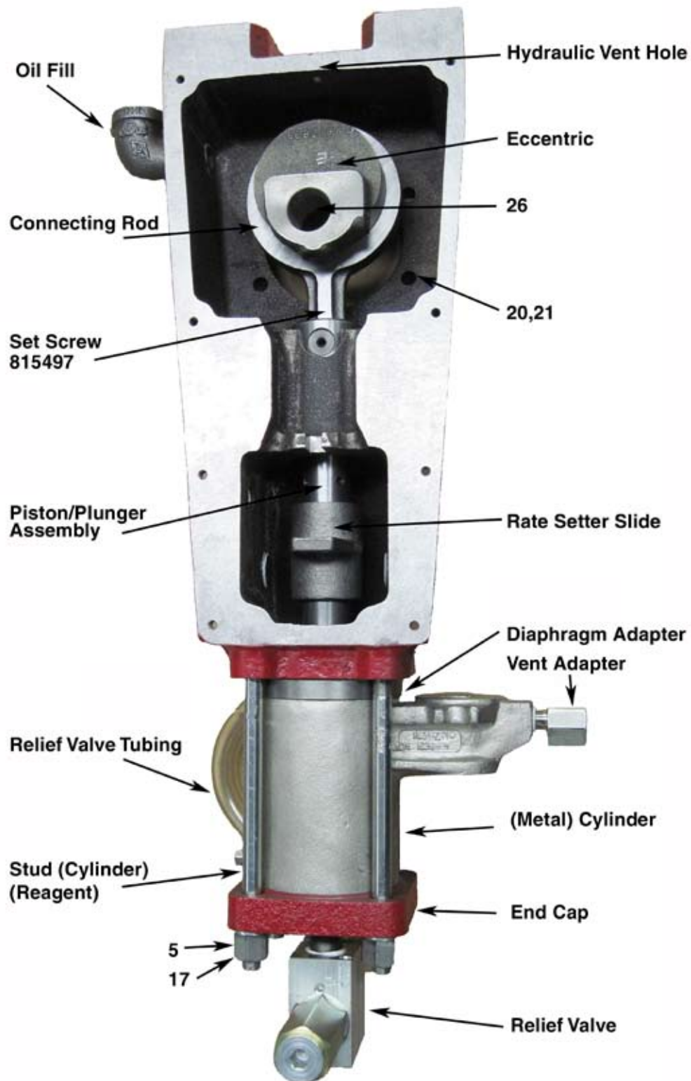
1" Plunger Hydraulic Assembly
